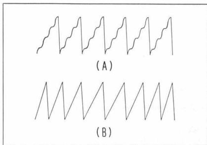
Fig. 6. Modulating waveforms for obtaining frequency-modulated offset carrier. (a) shows case where f - m deviation rate is greater than carrier offset, (b) where deviation rate is less than carrier offset.
