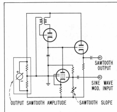
Fig. 5. Circuit for generating proper modulating waveform to obtain frequency-modulated offset carrier from twt.
