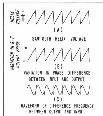
Fig. 4. Sketch of sawtooth modulating voltage applied to helix and its effect on output of twt. Discontinuity in (c) caused by sawtooth flyback has been exaggerated for illustrative purposes.
