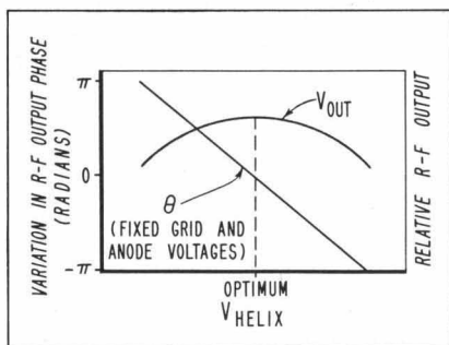
Fig. 3. Effect of helix voltage on phase shift and output voltage from twt.
