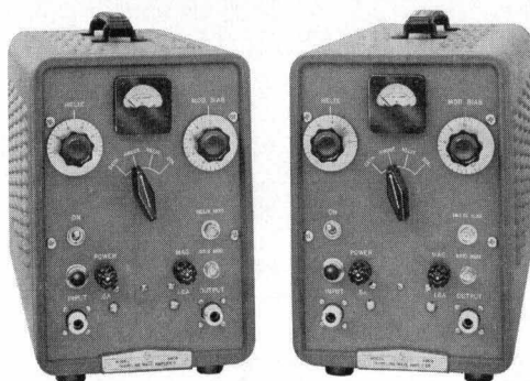
Fig. 1. New hp -492A and 494A Traveling-Wave Tube Amplifiers give more than 25 db of gain over 4-8 and 7-12.4 kmc ranges. Special modulation provision enable the amplifiers to be used to simulate doppler effects, to obtain amplitude-modulated signals or to form high-sensitivity linear detectors.
