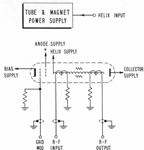
Fig. 2. Basic circuit arrangement of new amplifiers.
