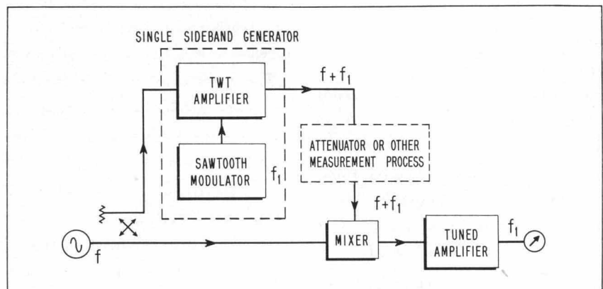
Fig. 8. Arrangement using twt and sawtooth modulator to form high-sensitivity linear homodyne detector for microwave signals.
