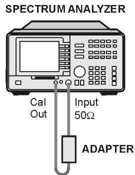
Figure 2-13 CAL FREQ Adjustment Routine Setup
