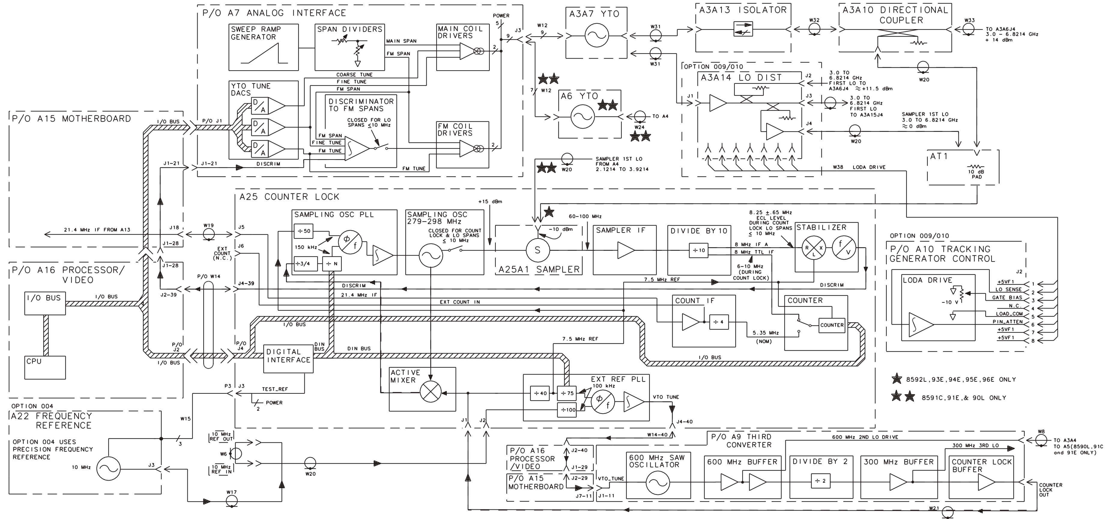
FOLDOUT 9-5. LO SECTION, BLOCK DIAGRAM
