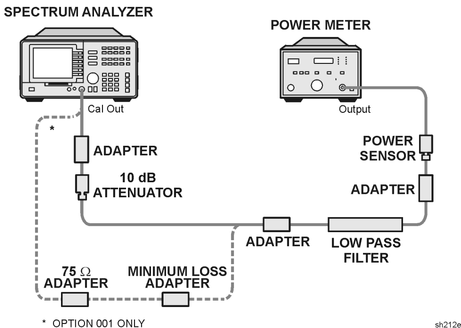
Figure 2-24 300 MHz Calibrator Amplitude Accuracy Test Setup
