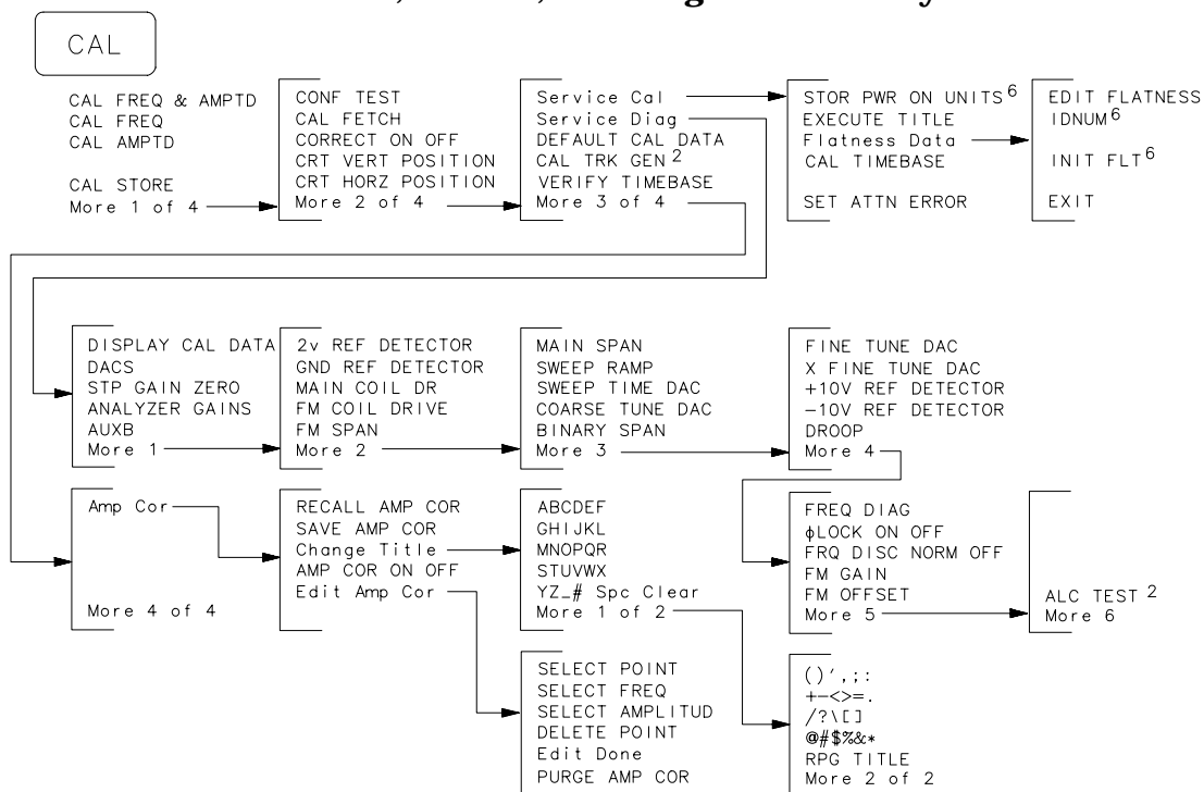
Figure 13-2 Calibration, Service, and Diagnostic Softkey Tree: 8591C
