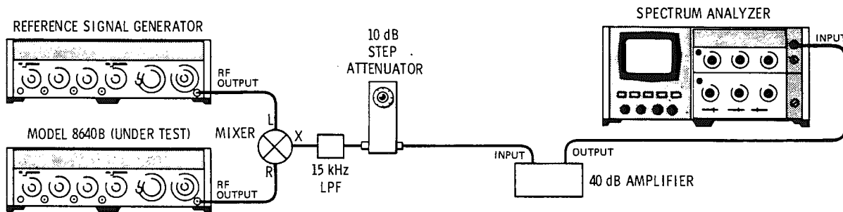
Figure 4-7. Single Sideband Broadband Noise Floor Test Setup
