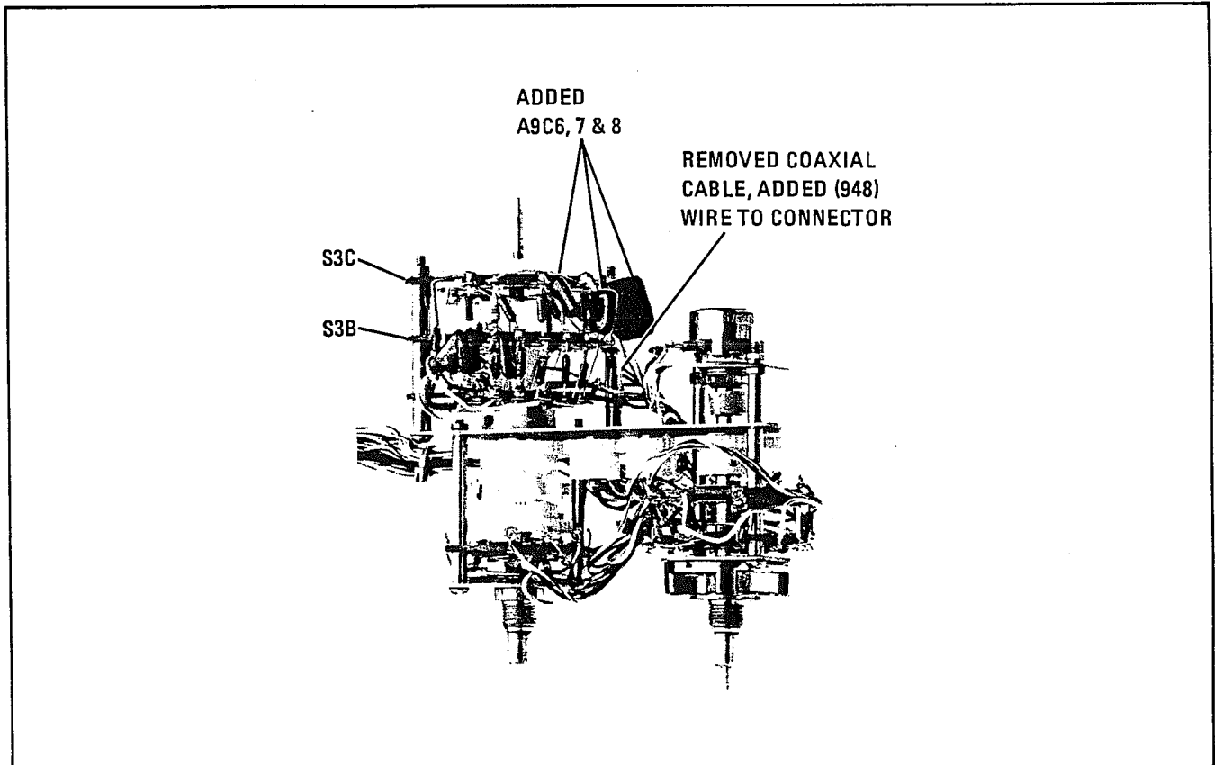
Figure 7-10. A9 Peak Deviation and Range Switch Modification
