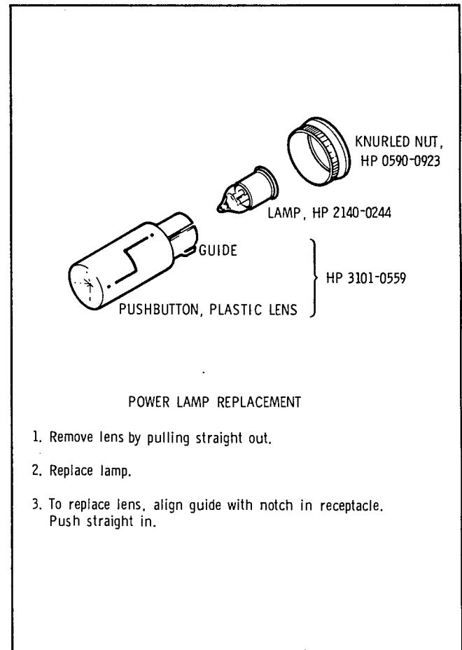
Figure 3-1. Lamp Replacement
