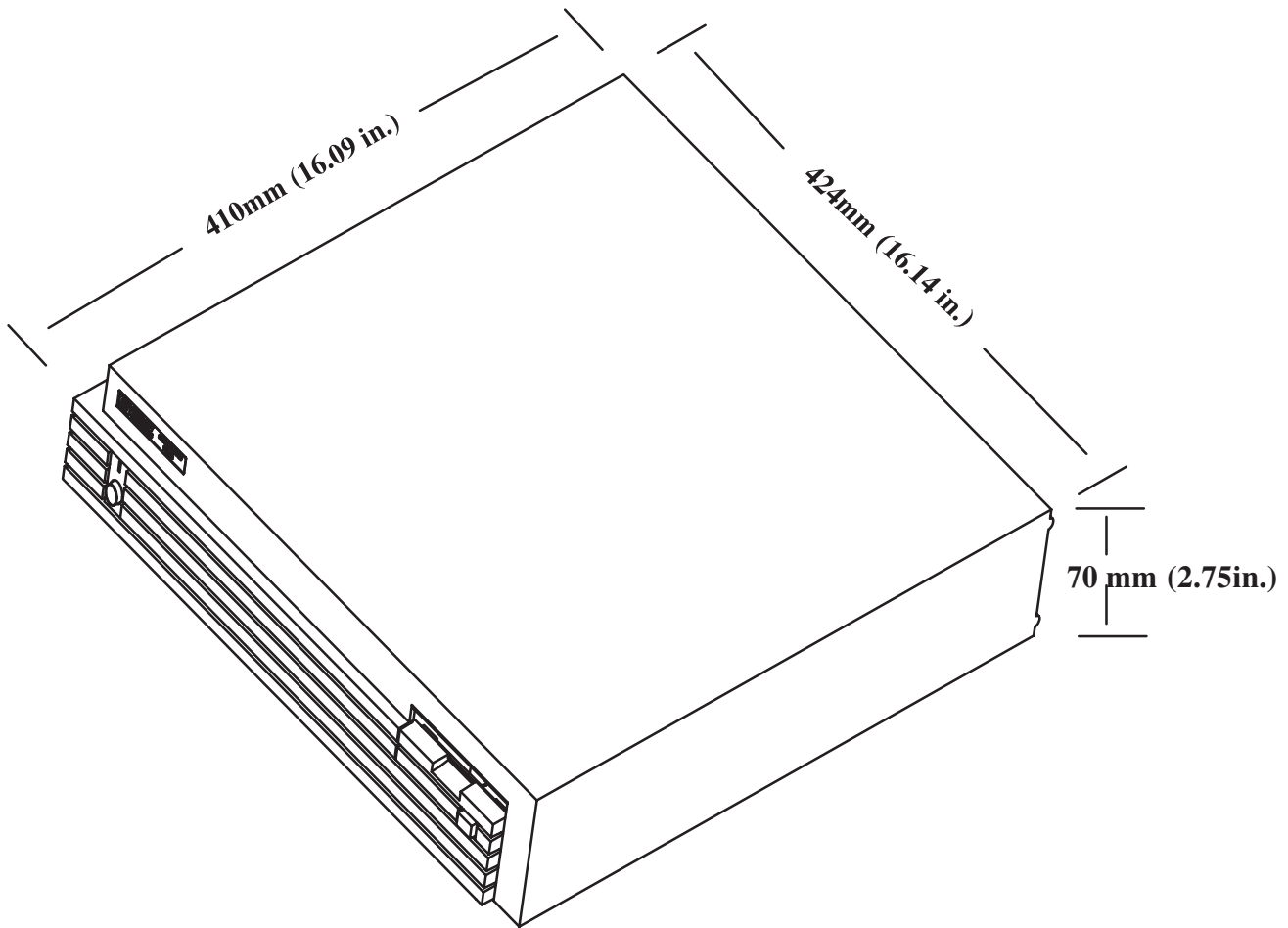
Figure 1–2. Chassis Dimensions
